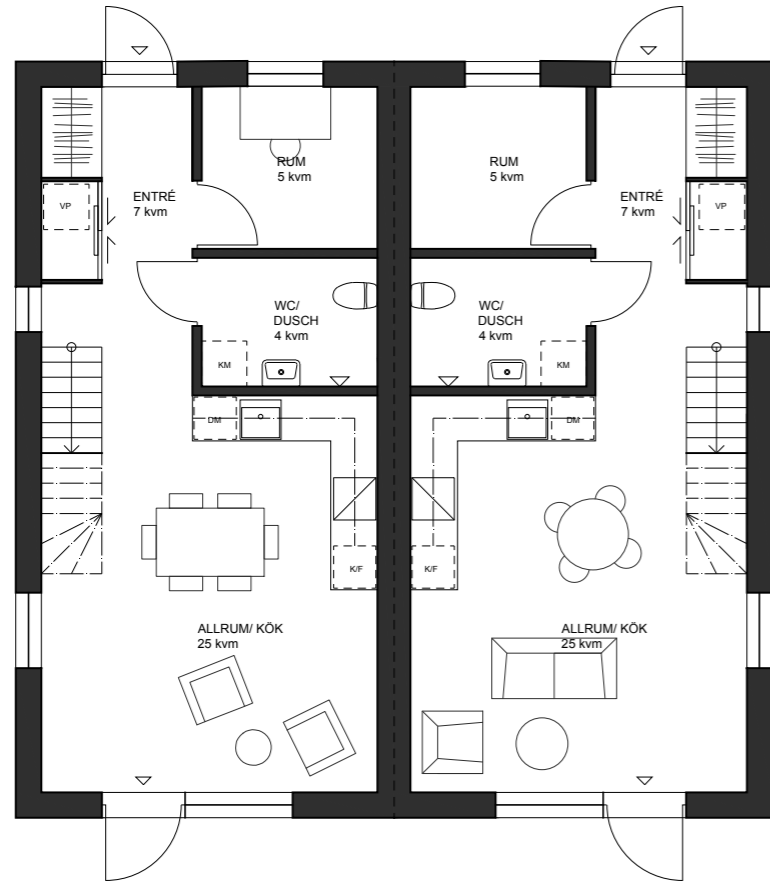
markplan
